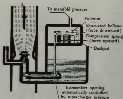
FIGURE 3-15. A pressure-operated economizer system.
